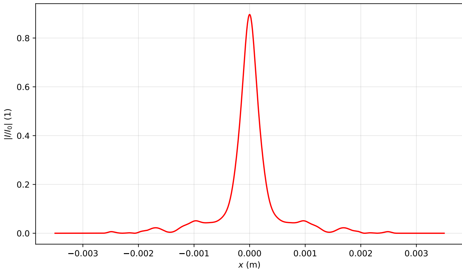
Intensity profile I(x, y = 0, z = 2.866)/I_0 , P_{in}=4.5P_{cr} , artificial time
